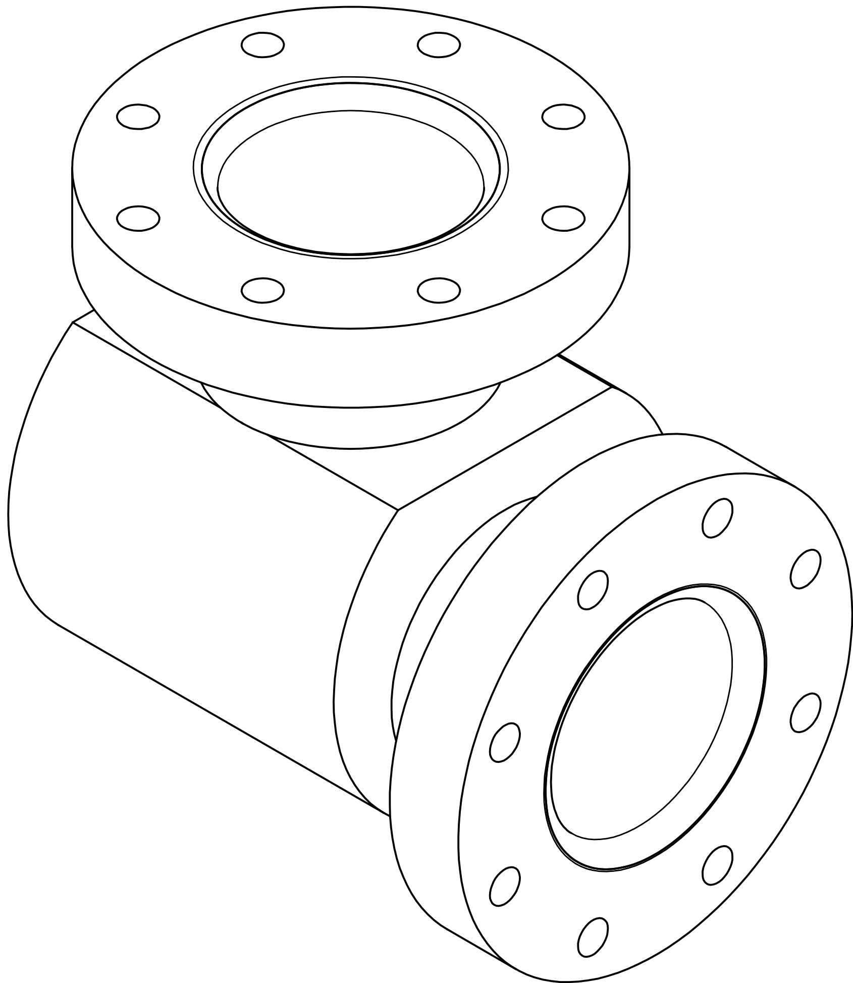
ISOMETRIC VIEW
